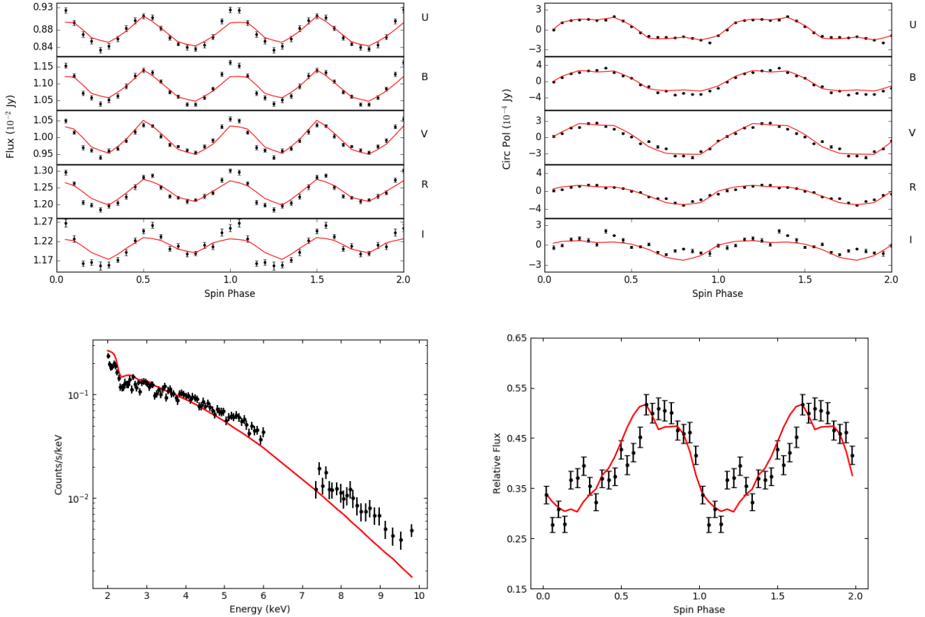
FIGURE 2. A good model of V405 Aur obtained by a simultaneous fitting of UBVRI light and polarization curves (top), X-rays spectrum, and hard X-ray light curve (bottom).
