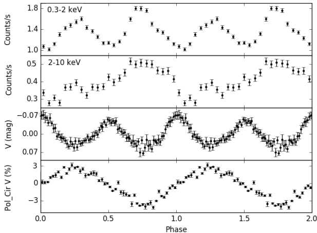
FIGURE 1. X-ray and optical light curves of V405 Aur folded on the optical ephemeris. From top to bottom, soft and hard X-ray data, photometry and circular polarimetry in V band.
